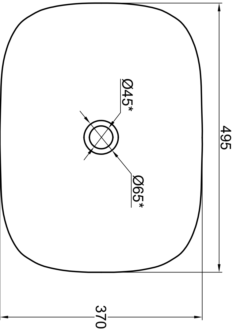
TOP VIEW
